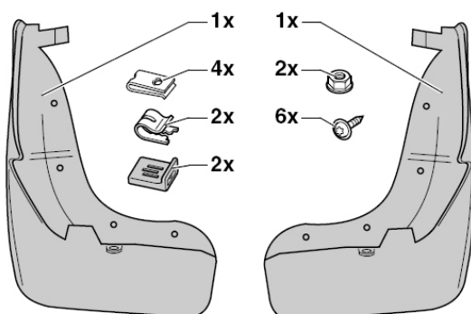
5K0 075 111 – Front
